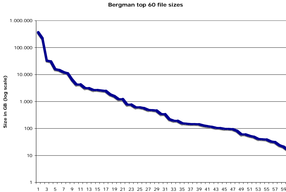
Figure 1: Distribution of file sizes in Bergman's Top 60
