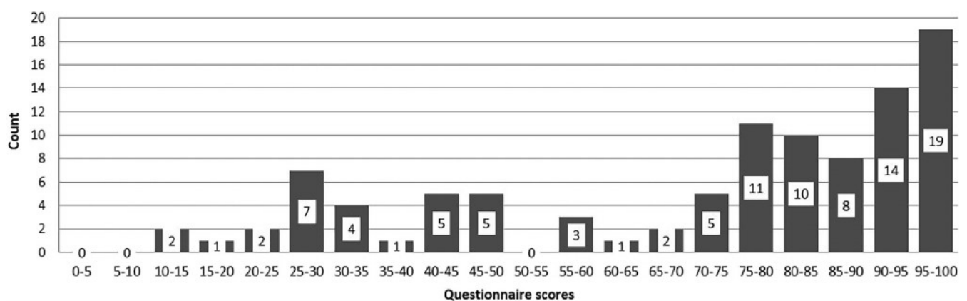
FIGURE 5 Questionnaire scores
